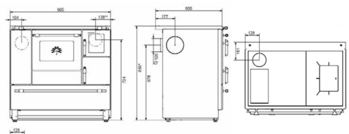
K 138CL links
