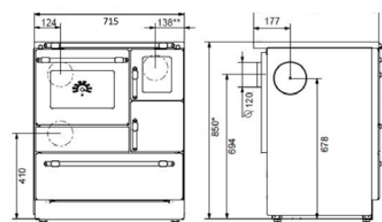
K 128F links
