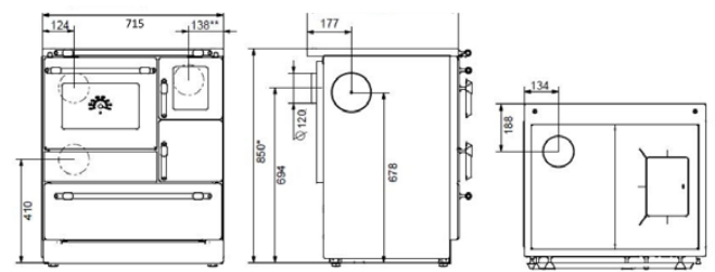
K 128CL links
